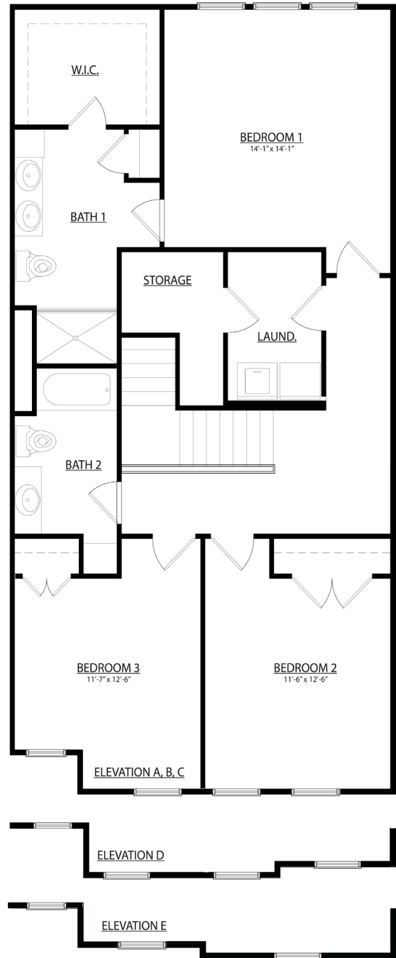
SECOND FLOOR PLAN 1113-1135 SQ. FT.
