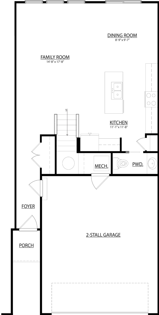
FIRST FLOOR PLAN 717-721 SQ. FT.
